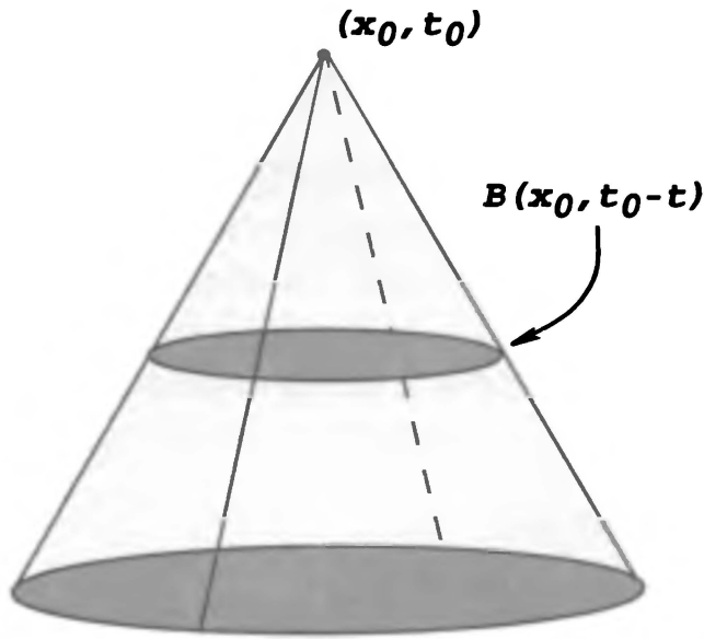
Cone of dependence
