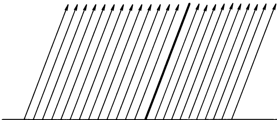
k -contact discontinuity
