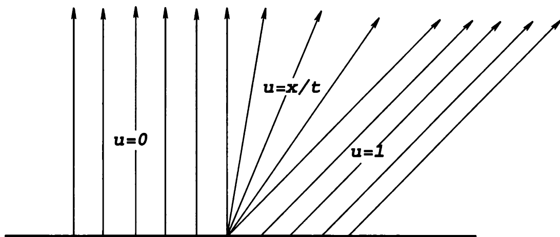
A “nonphysical” shock
