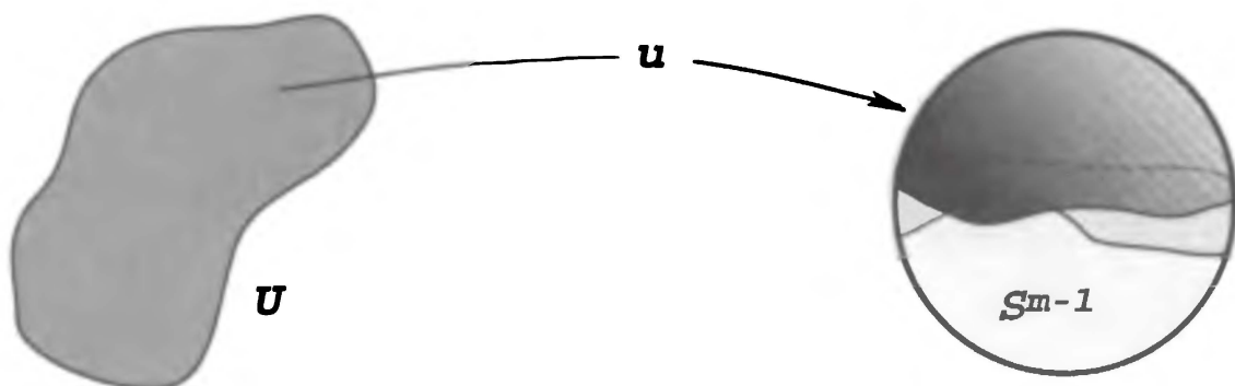
A harmonic map into a sphere
