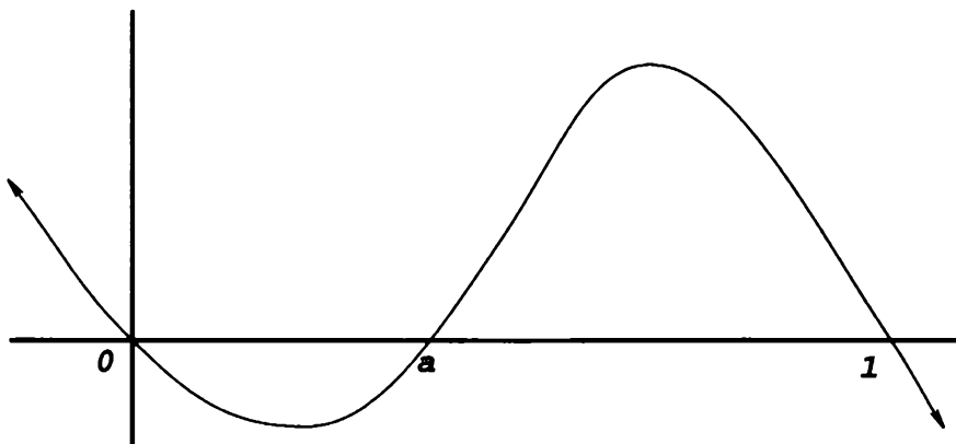
Graph of the function f
