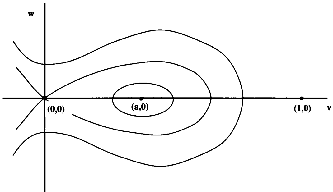
Level curves of E
