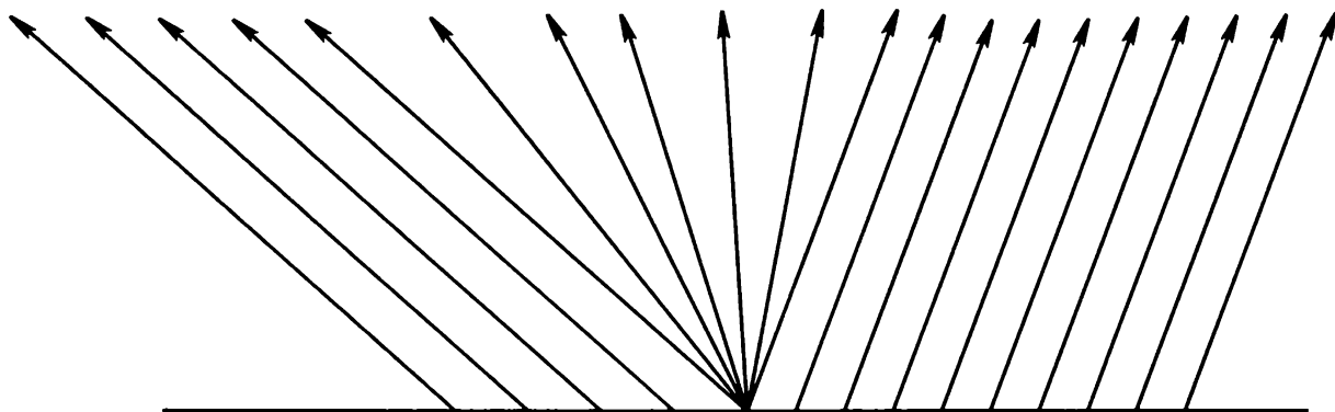
k -rarefaction wave
