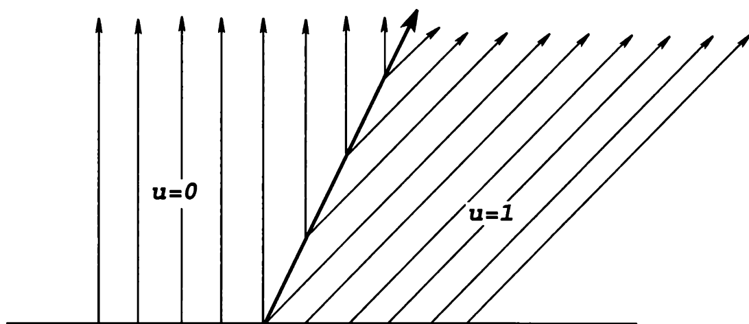
A “nonphysical” shock
