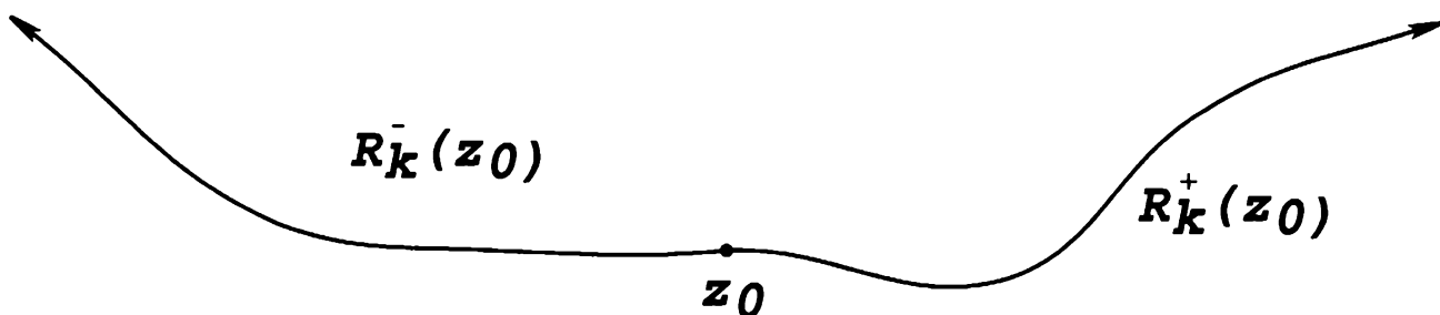
Two parts of the rarefaction curve
