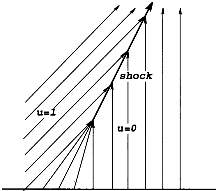
Formation of a shock
