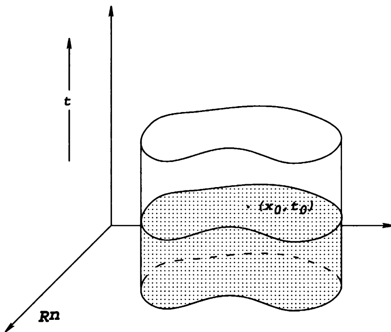
Strong maximum principle for the heat equation
