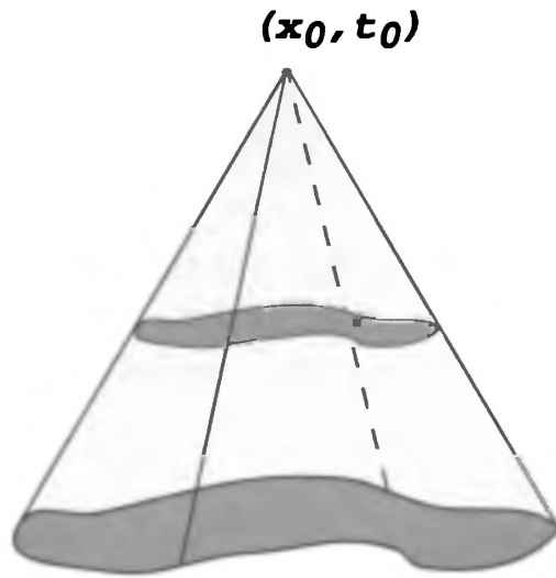
Domain of dependence
