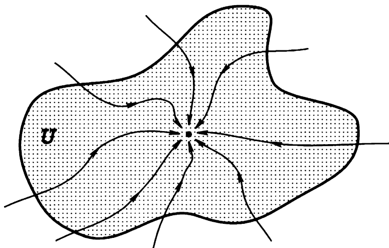
Case 1: flow to an attracting point
