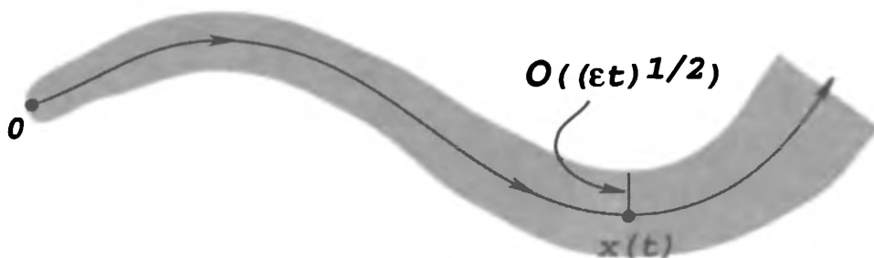
Flow of dye with diffusion
