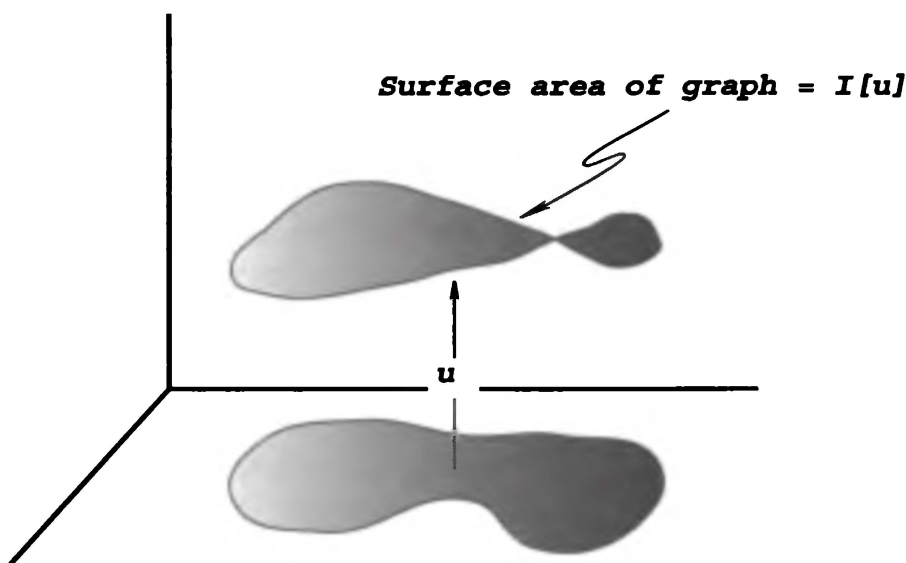
A minimal surface
